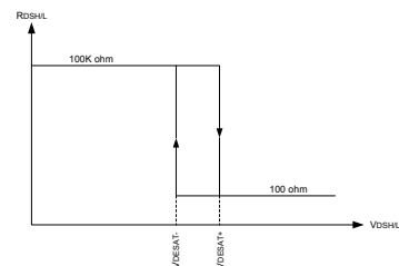
Figure 16: R_{DSH/L} Active Biasing
